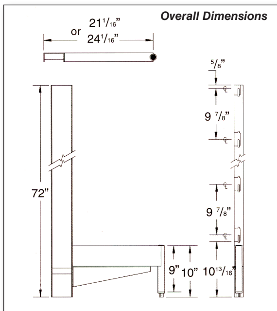
No corner posts maximizes storage
